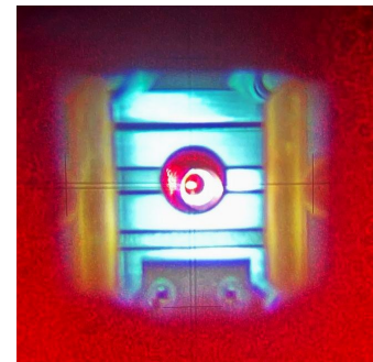
Lens upstream Cell Aperture
