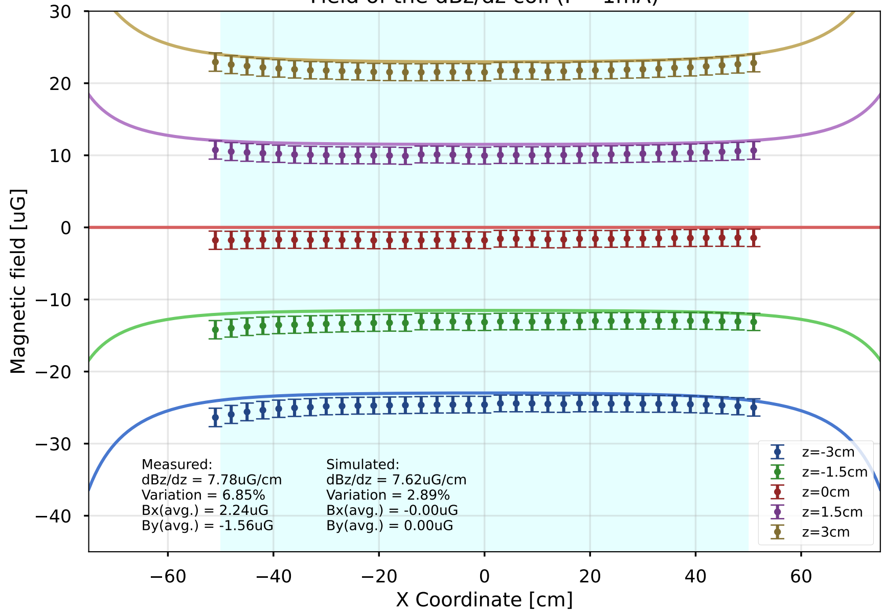
Field of the dBz/dz coil (I = 1mA)
