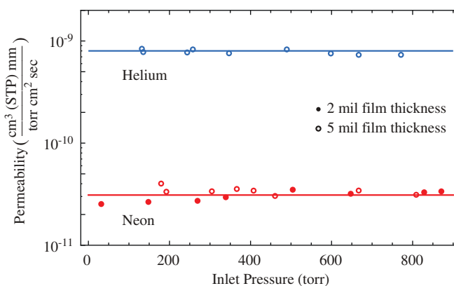
Fig. 3. The permeability of Kapton is independent of film thickness and inlet pressure, as shown with He and Ne.
